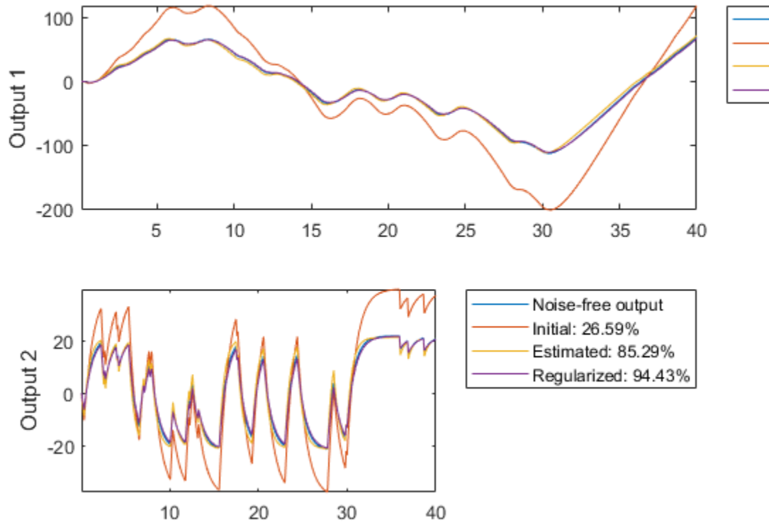
Figure 18: Noise-Free measured output and model outputs for initial, estimated and regularized models.
