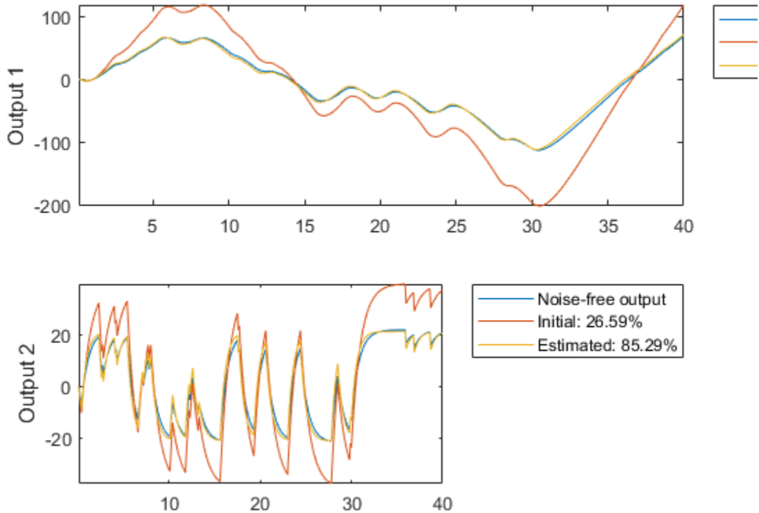
Figure 17: Noise-free output and model outputs for initial and estimated models.
