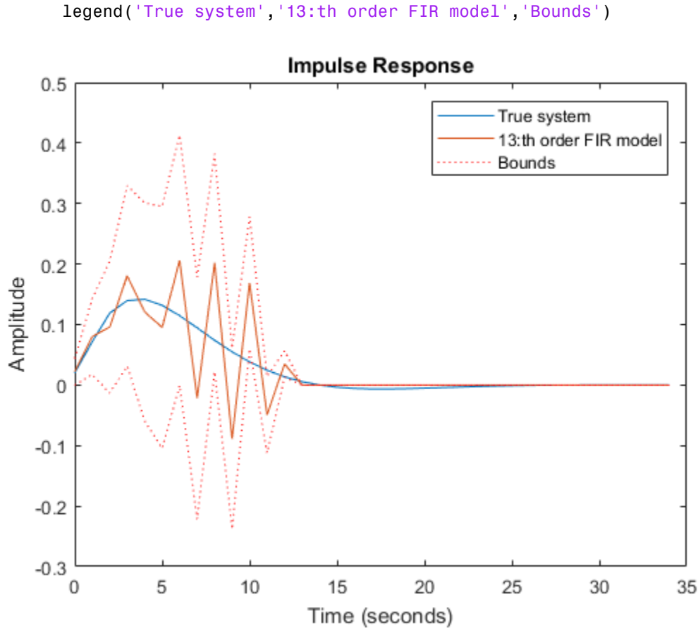
Figure 4: Estimated response with confidence bounds corresponding to 1 s.d.
